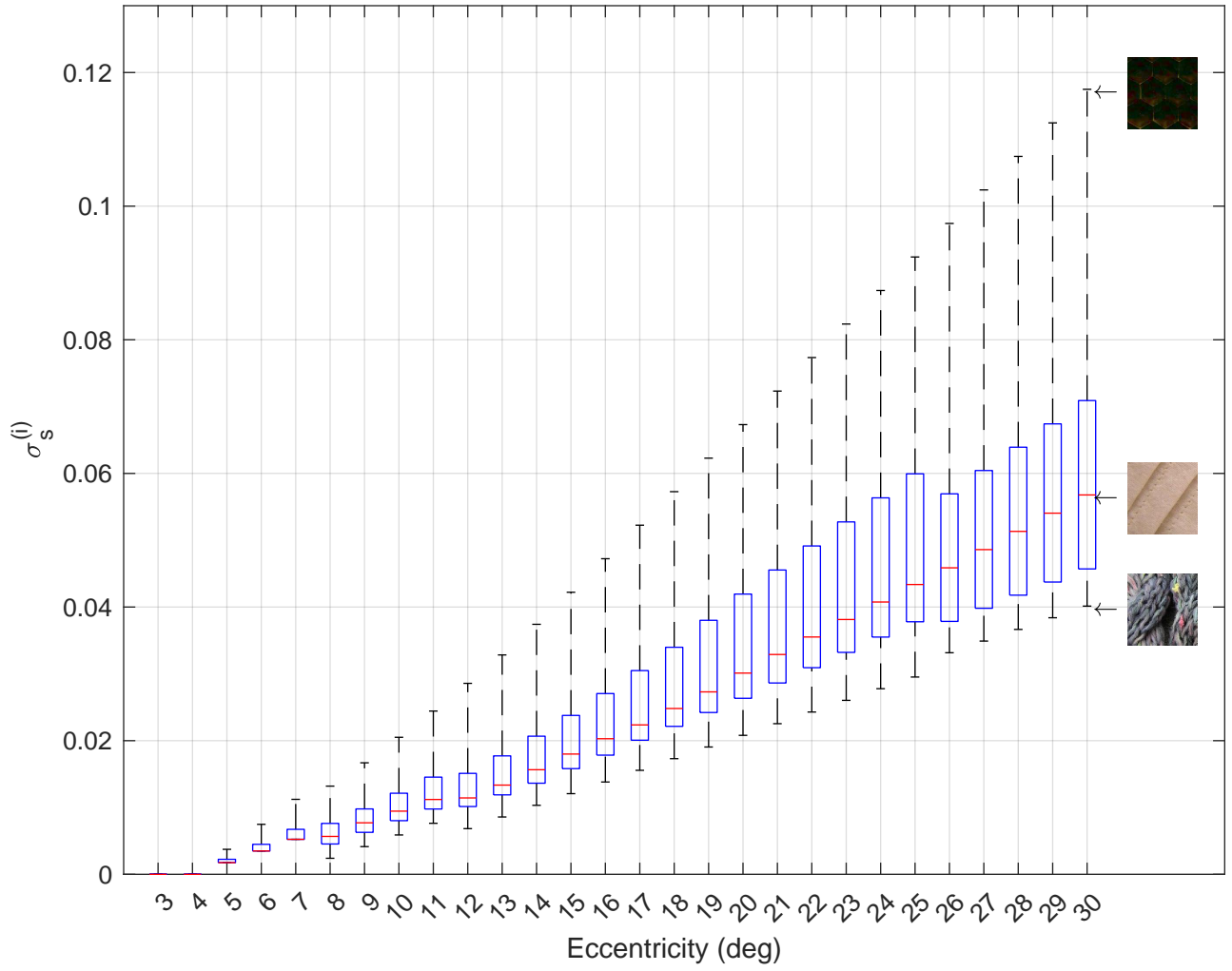
\sigma_s^{(i)} vs Eccentricity
